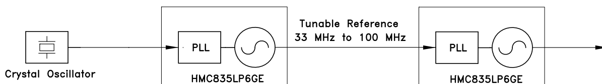
Figure 38. FRACTIONAL-N PLL WITH INTEGRATED VCO used as a tunable reference for HMC835LP6GE
