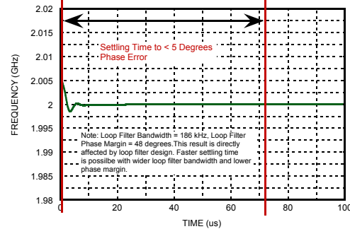
Figure 34. Frequency Settling After Frequency Change, Manual Calibration [23]
