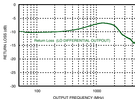
Figure 30. RF Output Return Loss Diff [21]
