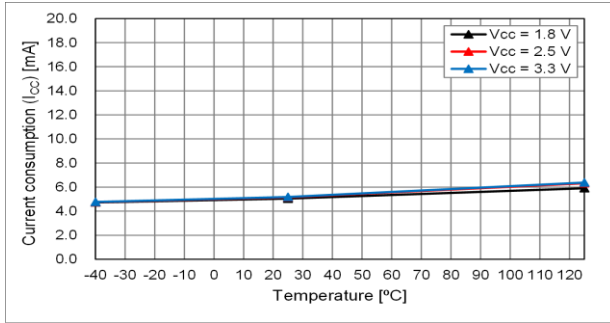
fo = 25 MHz
