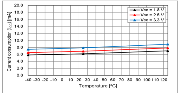
fo = 100 MHz
