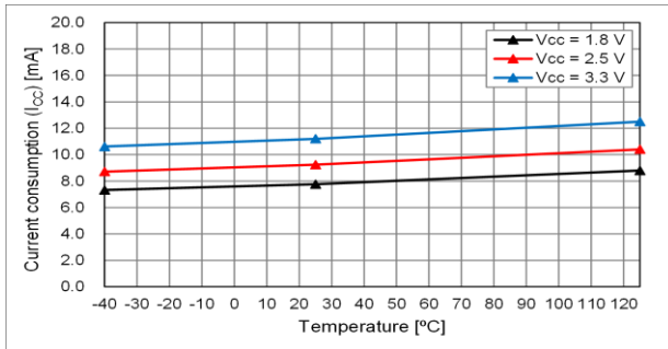
fo = 170 MHz
