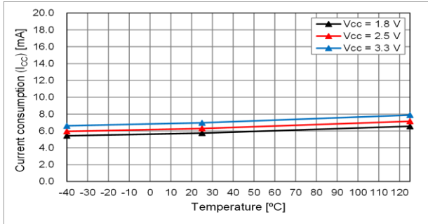
fo = 75 MHz
