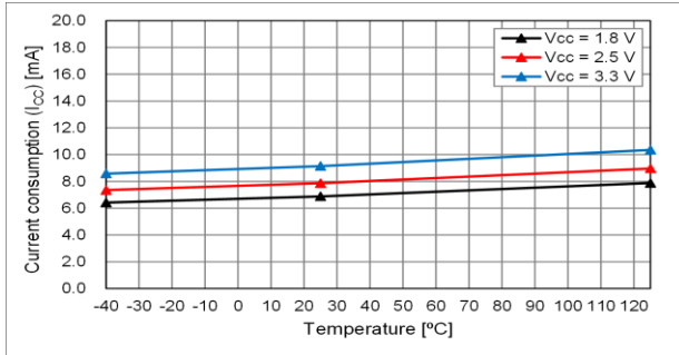
fo = 125 MHz
