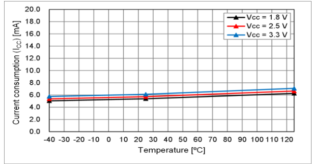
fo = 50 MHz
