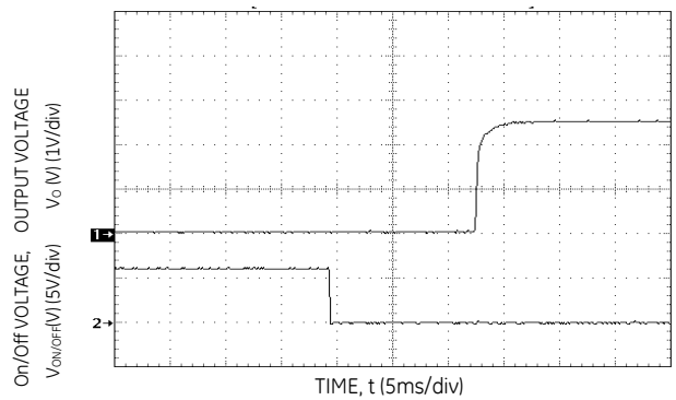
Figure 18. Typical Start-Up Using Remote On/Off, negative logic version shown.
