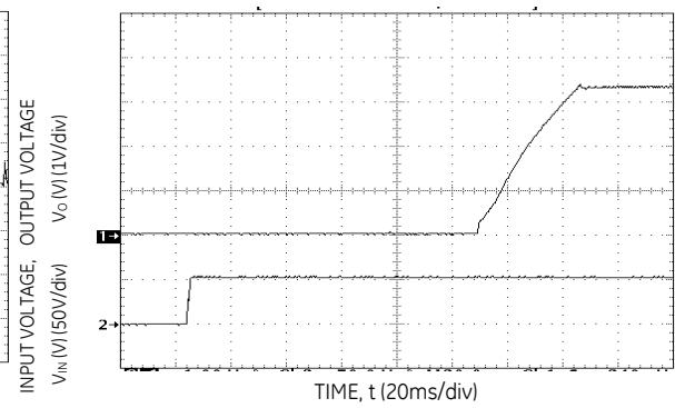
Figure 11. Typical Start-Up with application of V_{in} .
