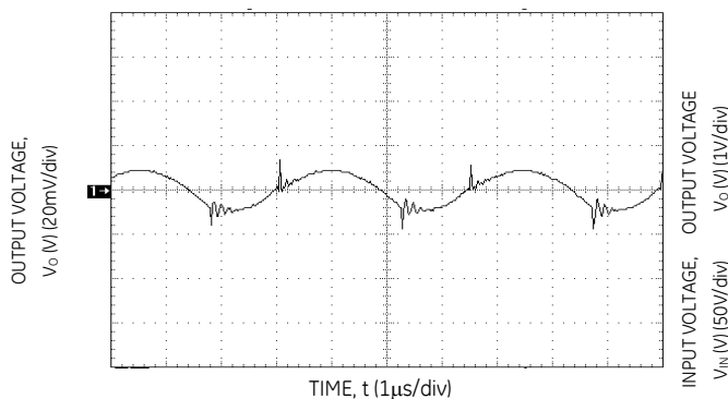
Figure 14. Typical Output Ripple and Noise.
