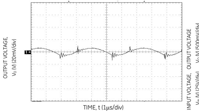
Figure 32. Typical Output Ripple and Noise.
