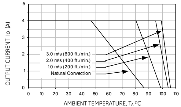
Figure 52. Derating Output Current versus Local Ambient Temperature and Airflow.
