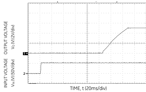
Figure 5. Typical Start-Up with application of V_{in} .
