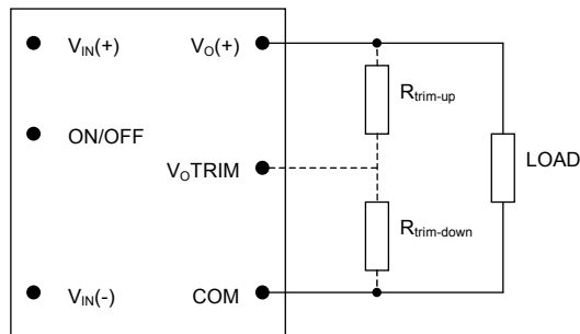
Figure 65. Circuit Configuration to Trim Output Voltage.
