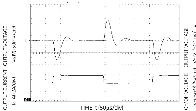
Figure 33. Transient Response to Dynamic Load Change from 50% to 75% to 50% of full load.
