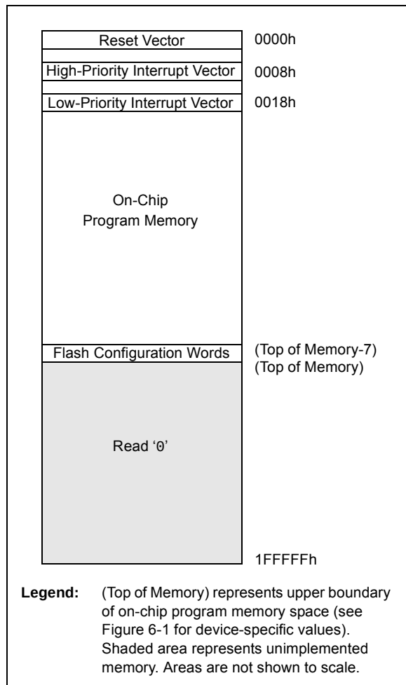
FIGURE 6-2: HARD VECTOR AND CONFIGURATION WORD LOCATIONS FOR PIC18F45J10 FAMILY DEVICES
