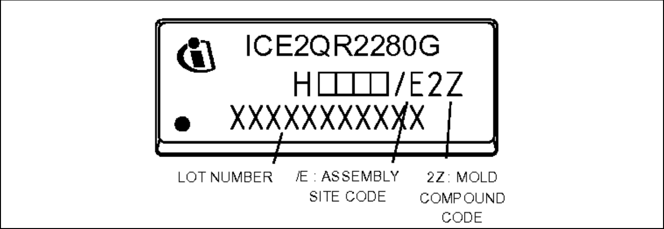
Figure 16 Marking for ICE2QR2280G
