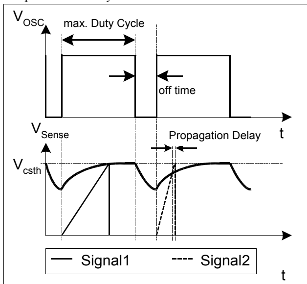
Figure 14 Dynamic Voltage Threshold V_{csth}
