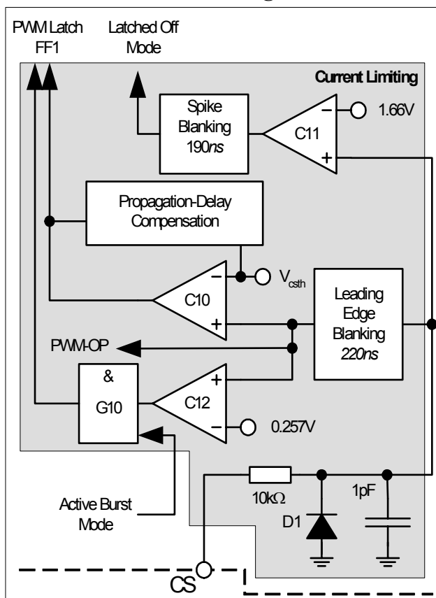
Figure 10 Current Limiting
