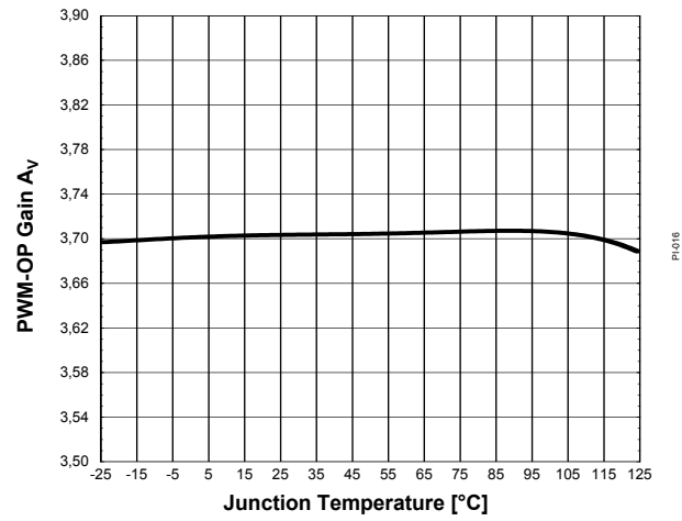
Figure 36 PWM-OP Gain A_V
