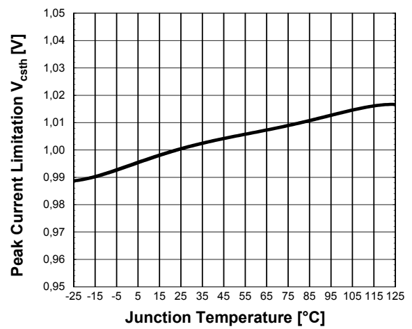
Figure 48 Peak Current Limitation V_{csth}
