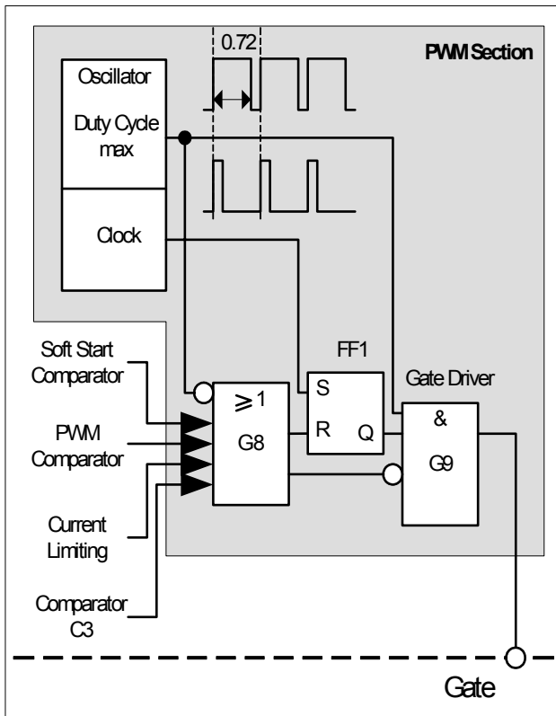
Figure 7 PWM Section
