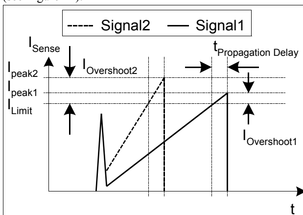
Figure 12 Current Limiting
