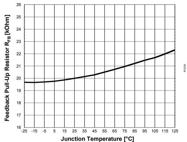
Figure 38 Feedback Pull-Up Resistor R_{FB}
