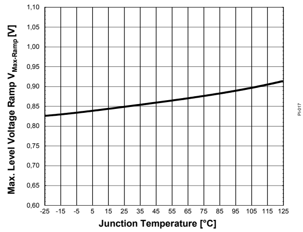
Figure 37 Max. Level Voltage Ramp V_{Max-Ramp}
