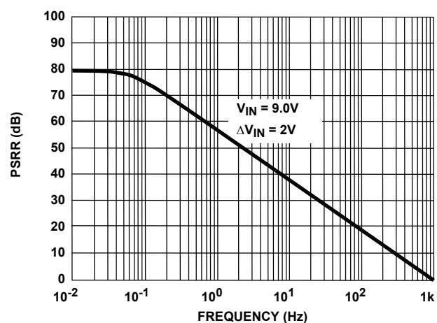
FIGURE 4. NPUT POWER SUPPLY REJECTION RATIO
