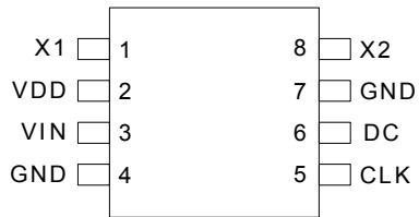
8-pin (150 mil) SOIC
