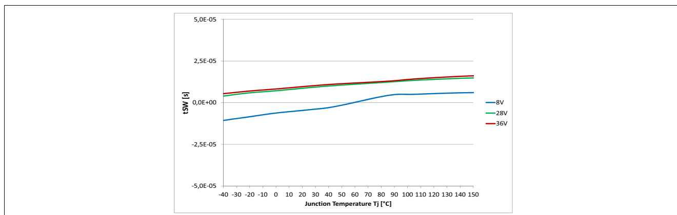
Figure 39 Turn ON / OFF matching \Delta t_{\text{SW}} = f(T_j; V_S) , R_L = 6 \Omega
