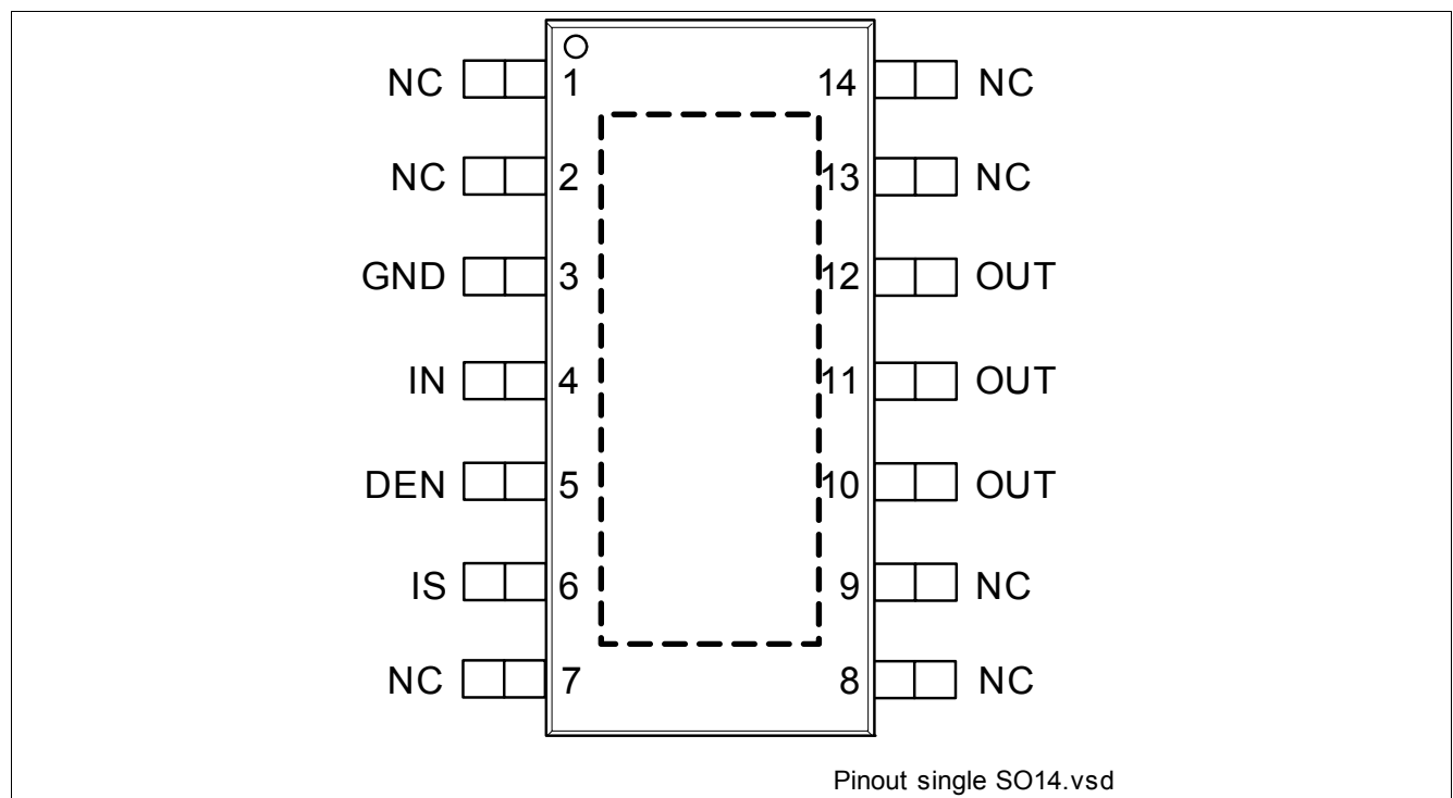
Figure 2 Pin Configuration
