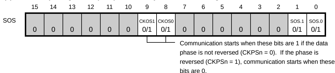
Figure 13-31. Example of Contents of Registers for Master Transmission of 3-Wire Serial I/O (CSISn) (1/2)
