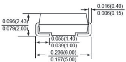
SMB/DO-214AA
