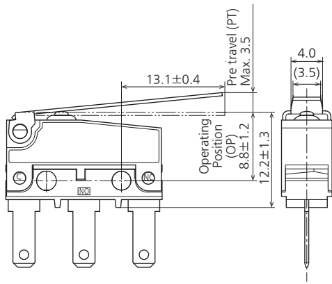
External dimensions
