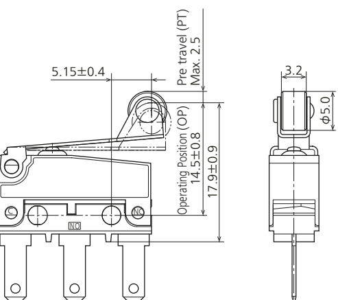
External dimensions
