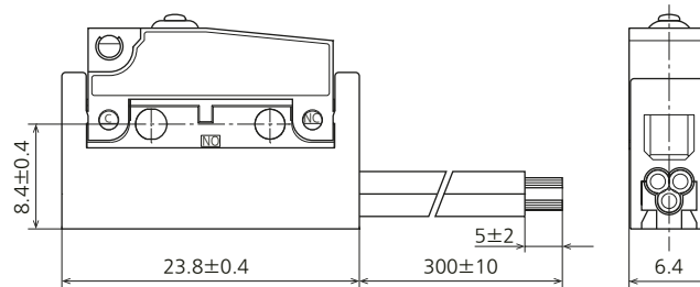
External dimensions
