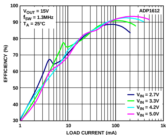
Figure 54. ADP1612 Efficiency vs. Load Current V_{OUT} = 15\text{ V} , f_{SW} = 1.3\text{ MHz}
