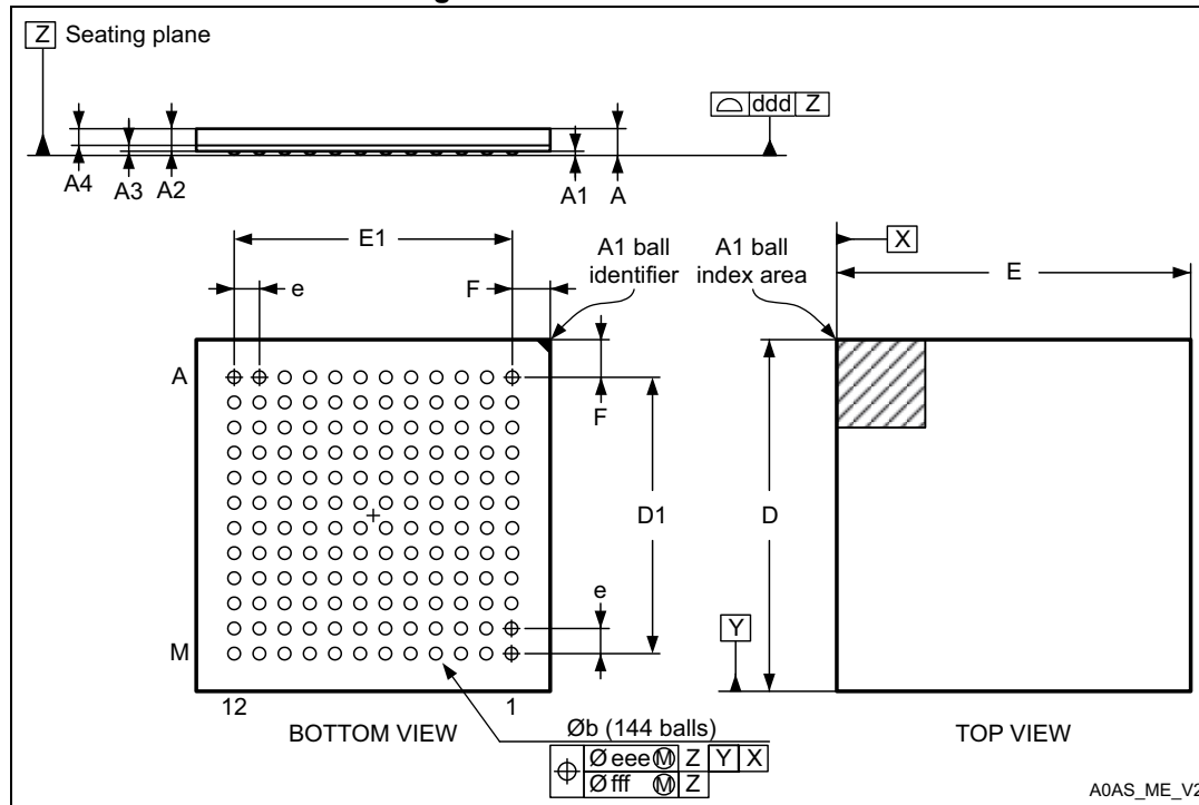
Figure 76. UFBGA144 outline
