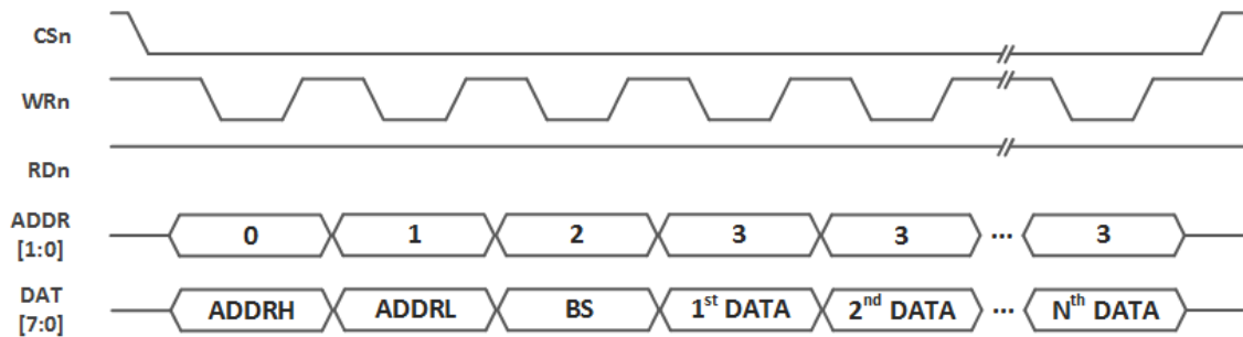
Figure 18 Parallel BUS N-Bytes Data Write Access
