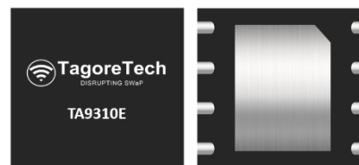
Figure 1.1 Device Image (8 Pin 5 x 6 x 0.75 mm DFN Package)
