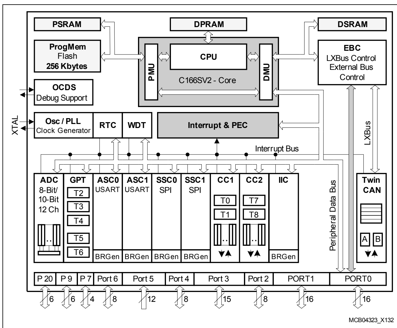
Figure 3 Block Diagram
