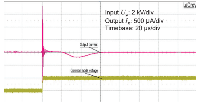
Figure 14: Detail of typical common mode perturbation (250 V step with 6 kV/μs, R_M = 100 \Omega )
