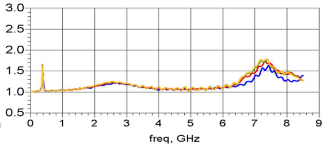
Figure 11.3.4: Mu1 vs Freq
