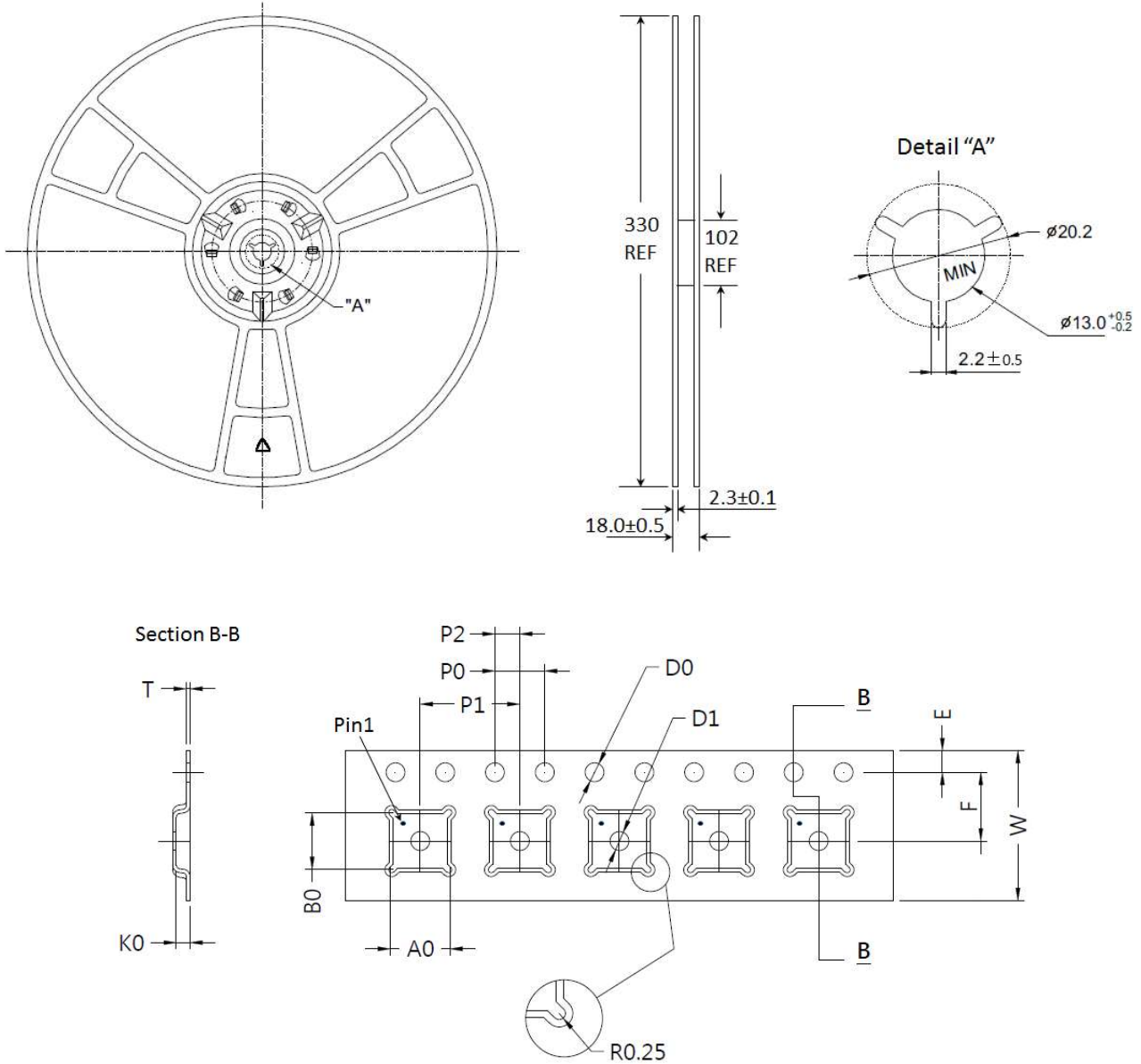
Figure 16.1 Tape and Reel Drawing
