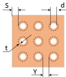
Figure 14.3 Thermal Via Pattern (Recommended Values: S \geq 0.15 mm; Y \geq 0.20 mm; d = 0.3 mm; Plating Thickness t = 25 \mu m or 50 \mu m)
