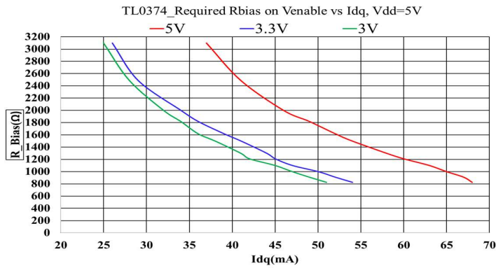
Figure 11.3.5: Rbias on Venable vs Idq
