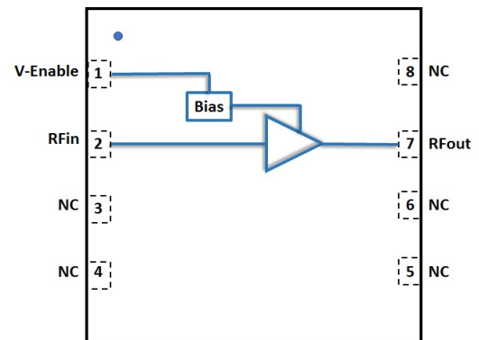
Figure 3.1 Function Block Diagram (Top View)
