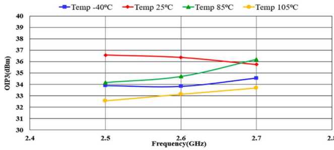
Figure 11.3.3: Output IP3 vs Freq
