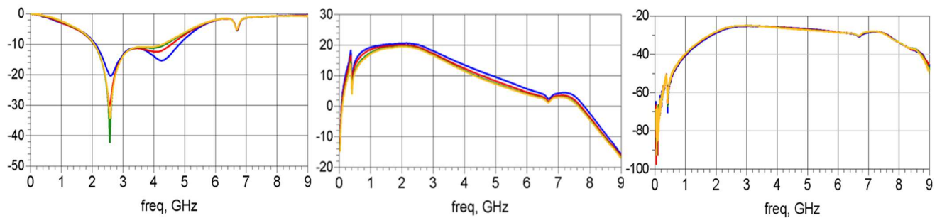
Figure 11.2.1: S11(IREL) vs Freq
