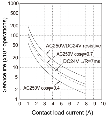
Life curve
