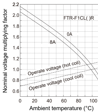
Operating range
