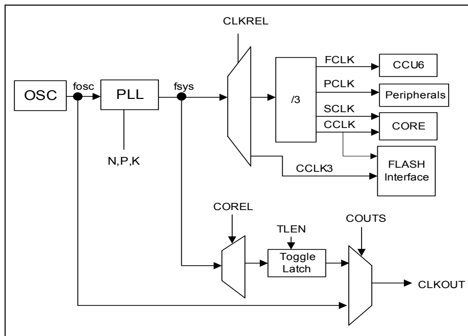
Figure 25 Clock Generation from f_{\text{sys}}
