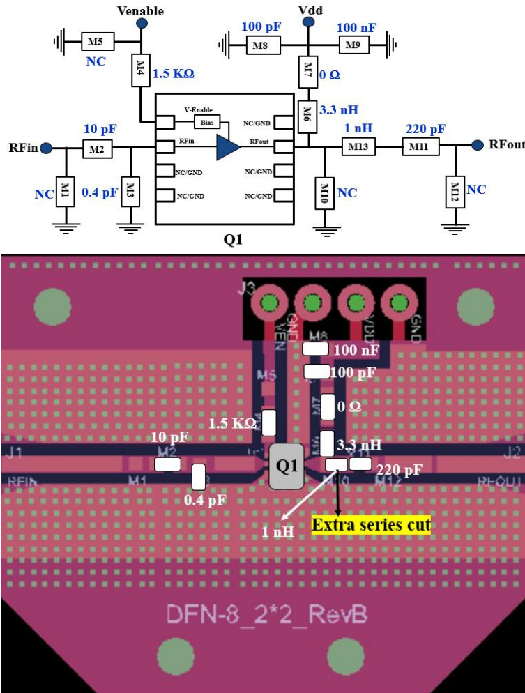
Figure 10.1 Schematic and EVB layout of the 3300-3800 MHz EVB-A
