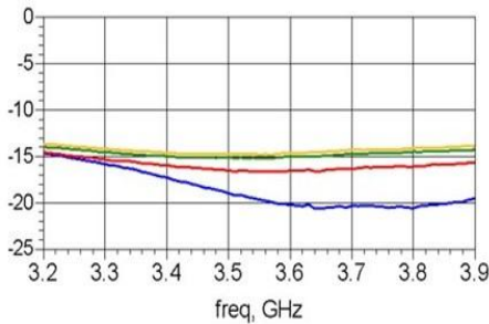
Figure 11.1.1: S11(TRL) vs Freq
