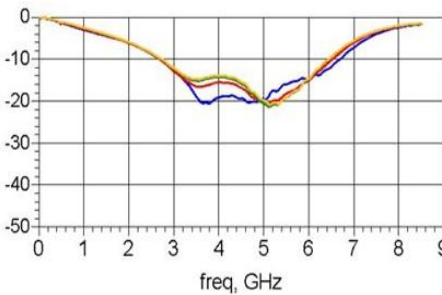
Figure 11.2.1: S11(TRL) vs Freq
