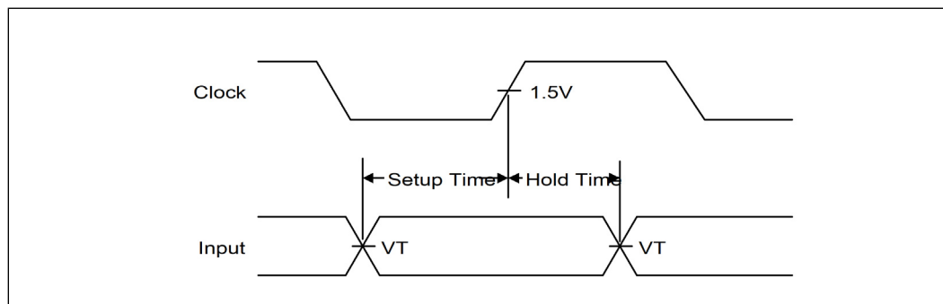
Figure 10-19. Pulse Width
