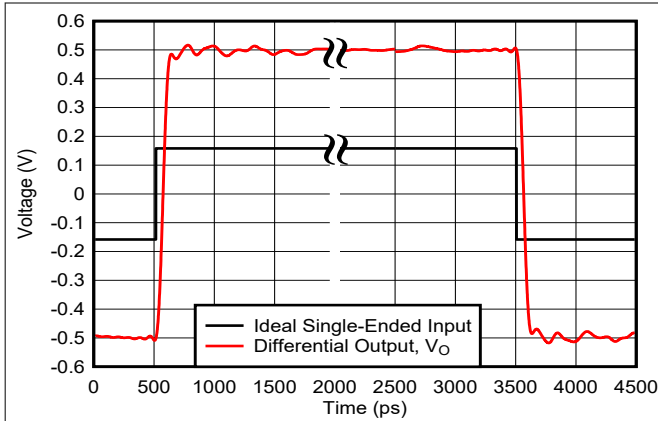
Figure 6-31. Step Response
