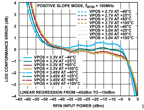
Figure 7. Log Conformance Error vs. P_{RFIN} Over Temperature and VPOS at 100 MHz, Positive Slope Mode
