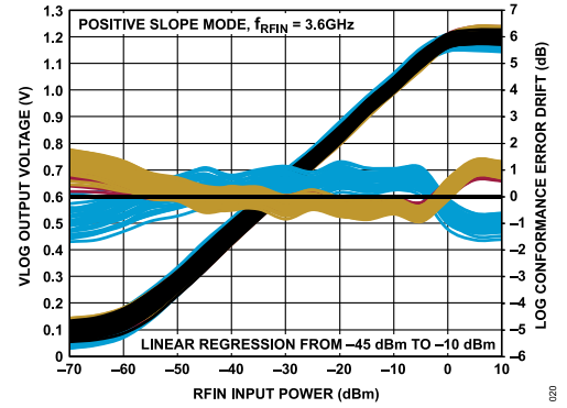
Figure 20. Distribution of V_{LOG} and Log Conformance Error Drift with Respect to 25°C vs. P_{RFIN} at 3.6 GHz, Positive Slope Mode
