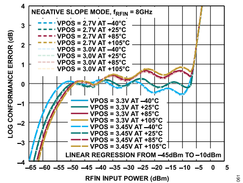
Figure 61. Log Conformance Error vs. P_{RFIN} Over Temperature and VPOS at 8 GHz, Negative Slope Mode
