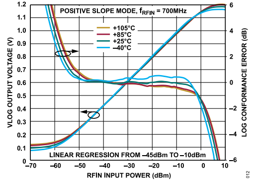
Figure 12. V_{VLOG} and Log Conformance Error vs. P_{RFIN} Over Temperature at 700 MHz, Positive Slope Mode
