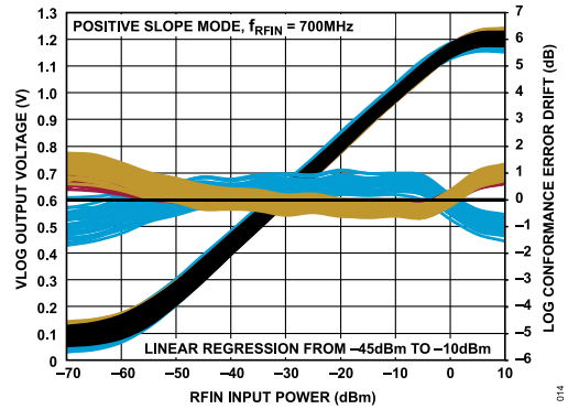
Figure 14. Distribution of V_{VLOG} and Log Conformance Error Drift with Respect to 25°C vs. P_{RFIN} at 700 MHz, Positive Slope Mode
