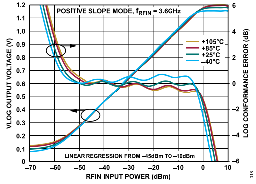
Figure 18. V_{LOG} and Log Conformance Error vs. P_{RFIN} Over Temperature at 3.6 GHz, Positive Slope Mode
