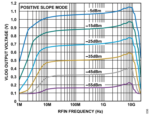
Figure 36. V_{LOG} vs. f_{RFIN} in Log Scale Over Input Powers, Positive Slope Mode
