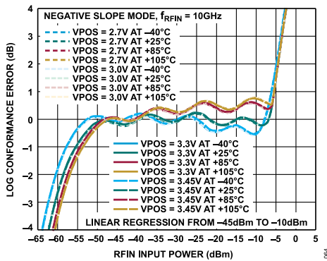
Figure 64. Log Conformance Error vs. P_{RFIN} Over Temperature and VPOS at 10 GHz, Negative Slope Mode
