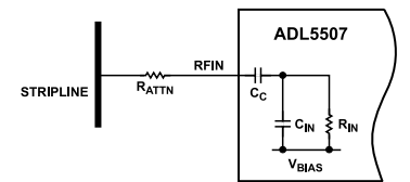
Figure 86. Series Attenuation Method for Input Coupling
