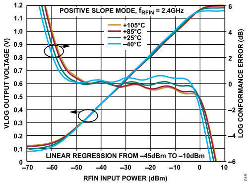
Figure 15. V_{LOG} and Log Conformance Error vs. P_{RFIN} Over Temperature at 2.4 GHz, Positive Slope Mode
