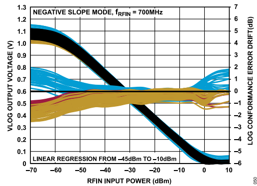
Figure 50. Distribution of V_{VLOG} and Log Conformance Error Drift with Respect to 25°C vs. P_{RFIN} at 700 MHz, Negative Slope Mode
