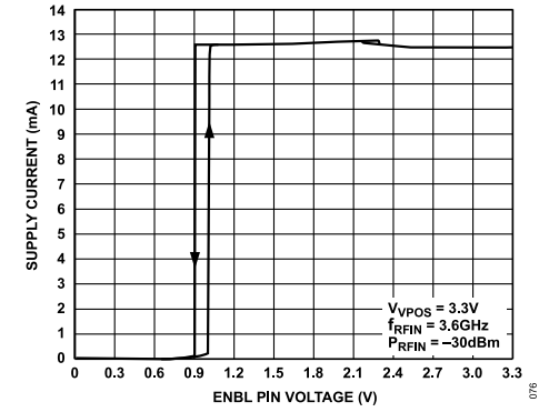
Figure 74. Supply Current vs. ENBL Pin Voltage
