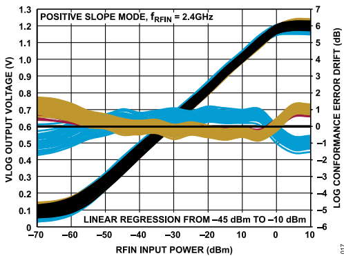
Figure 17. Distribution of V_{LOG} and Log Conformance Error Drift with Respect to 25°C vs. P_{RFIN} at 2.4 GHz, Positive Slope Mode
