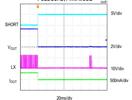
MAXM17904 OUTPUT SHORT IN STEADY STATE V_{IN} = 12V , FIXED V_{OUT} = 3.3V , FULL LOAD, PWM MODE
