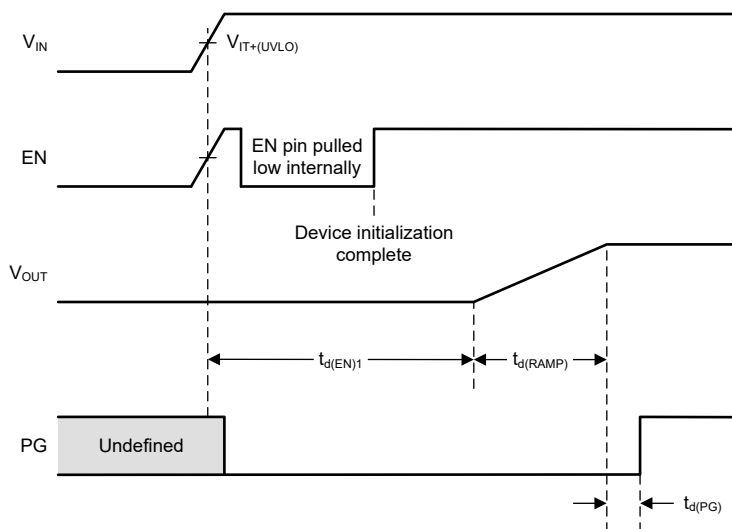
Figure 7-11. Start-Up Timing When EN is Pulled Up to V_{\text{IN}}
