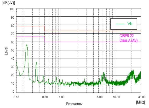
Conduction Noise ( V_{IN} = 48V, I_{OUT} = 2A, T_a = +25degC ) with External Input Filter
