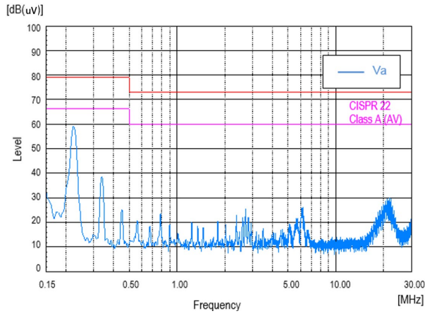
Conduction Noise ( V_{IN} = 48V, I_{OUT} = 2A, T_a = +25degC ) with External Input Filter
