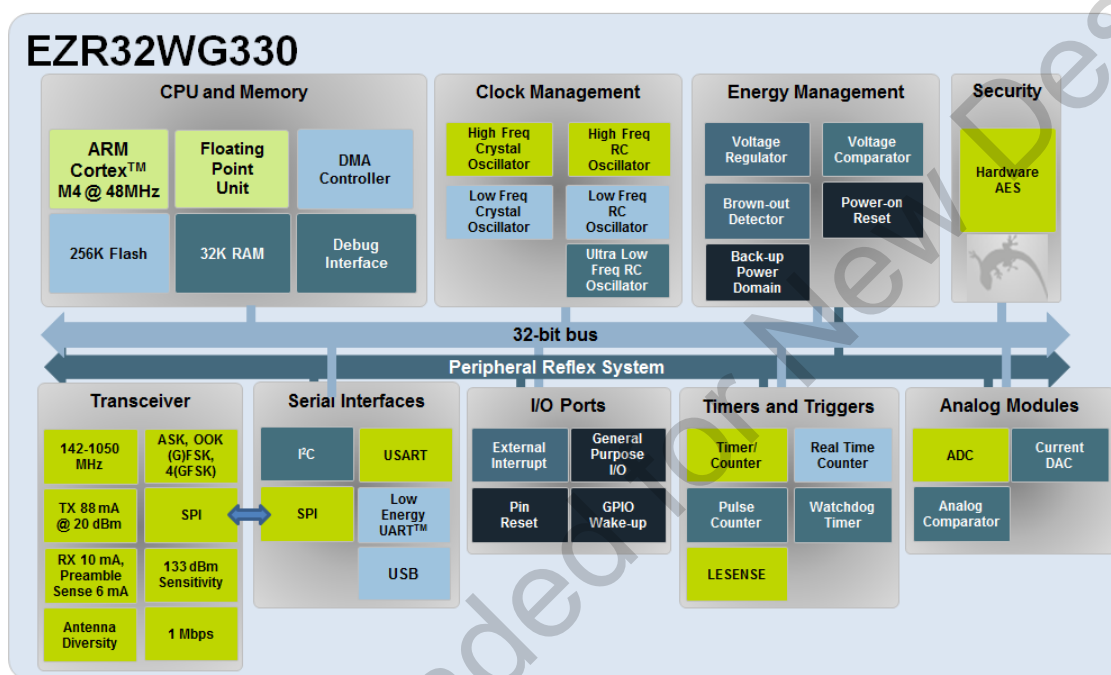
Figure 3.1. Block Diagram
