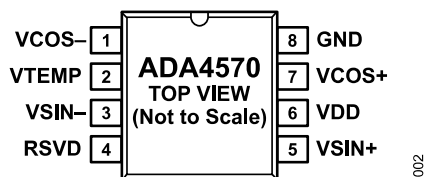
Figure 2. Pin Configuration
