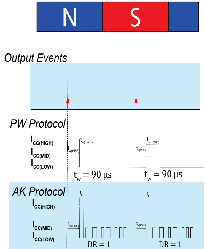
Figure 9: Output Timing Example
