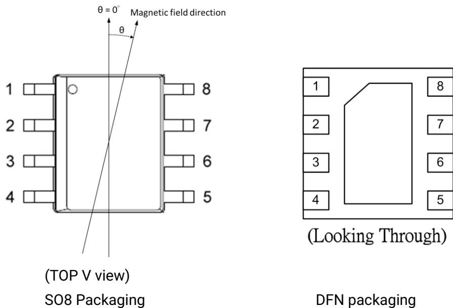
Figure 3. Pin Assignments
