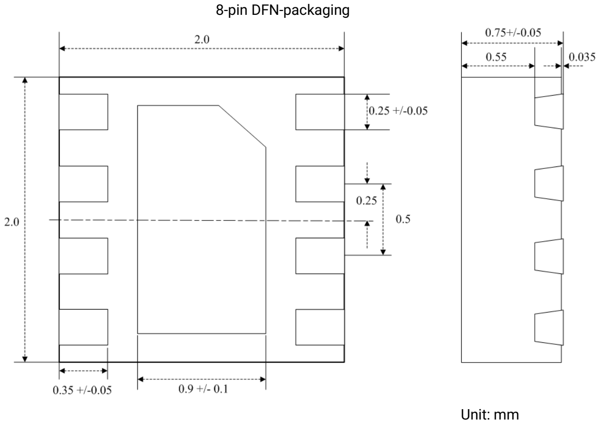
Figure 3. Package dimensions
