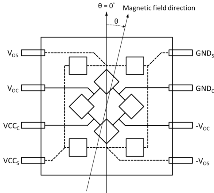
Figure 1. Circuit diagram and definition of magnetic field direction
