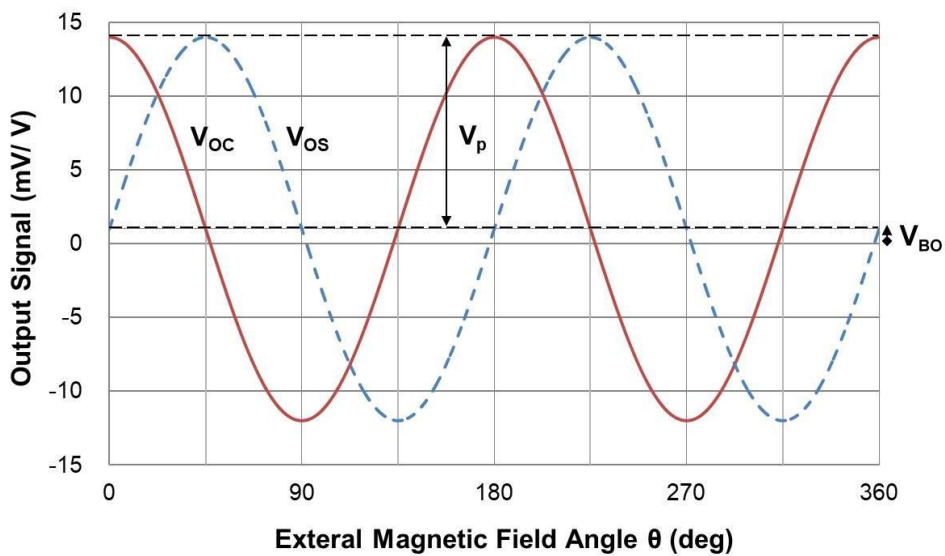
Figure 2. Sensor output as a function of the angle \theta
