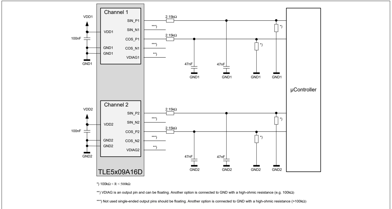
Figure 14 Application circuit for the TLE5x09A16(D) for partial diagnostics with pull-down resistors in single-ended output mode; positive output channels used
