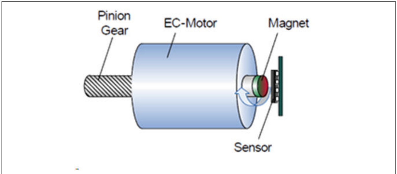
Figure 1 A usual application for TLE5x09A16(D) is the electrically commutated motor
