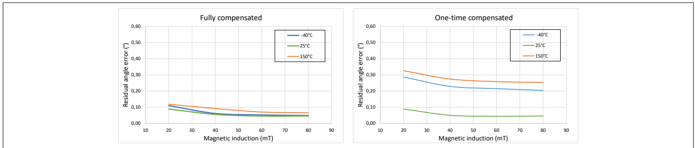
Figure 21 Typical residual angle error of fully and one-time compensated AMR sensor for differential output at different temperatures (measured at 0 h); one-time compensation is calibrated at T = 25^{\circ}\text{C} and B = 40\text{ mT} ; TLE5309D derivative with TCO (Temperature Compensation Offset) and 3.3 V supply voltage is used
