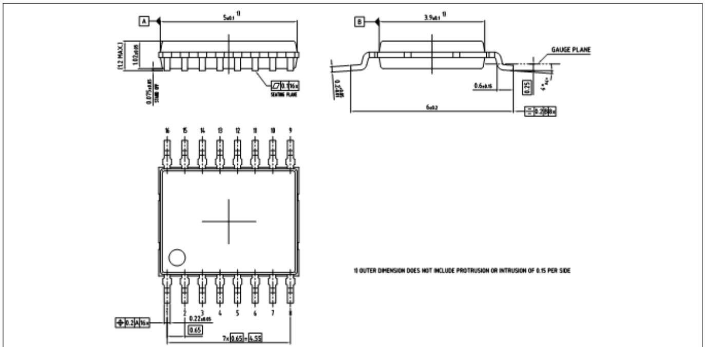
Figure 22 Package dimensions
