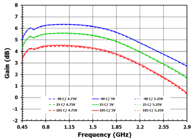
Figure 8. Gain, DSA1 = 6dB, Bypass ON
