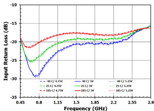
Figure 48. S11, DSA1 = 6dB, Bypass OFF
