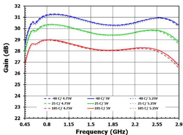
Figure 5. Gain, DSA0 = 6dB, Bypass OFF
