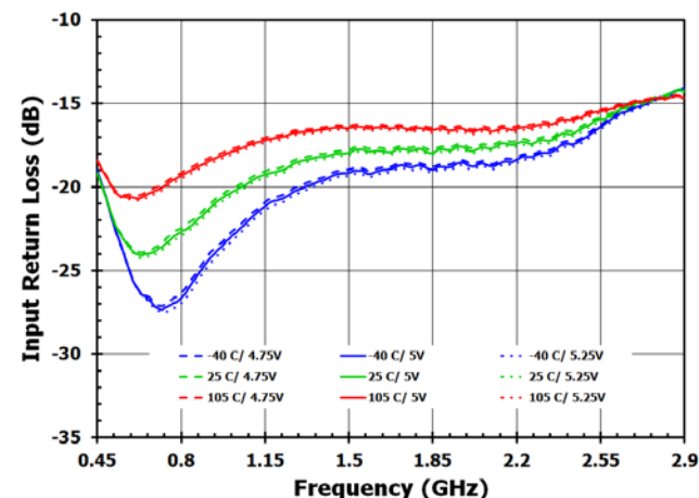
Figure 50. S11, DSA2 = 5dB, Bypass OFF
