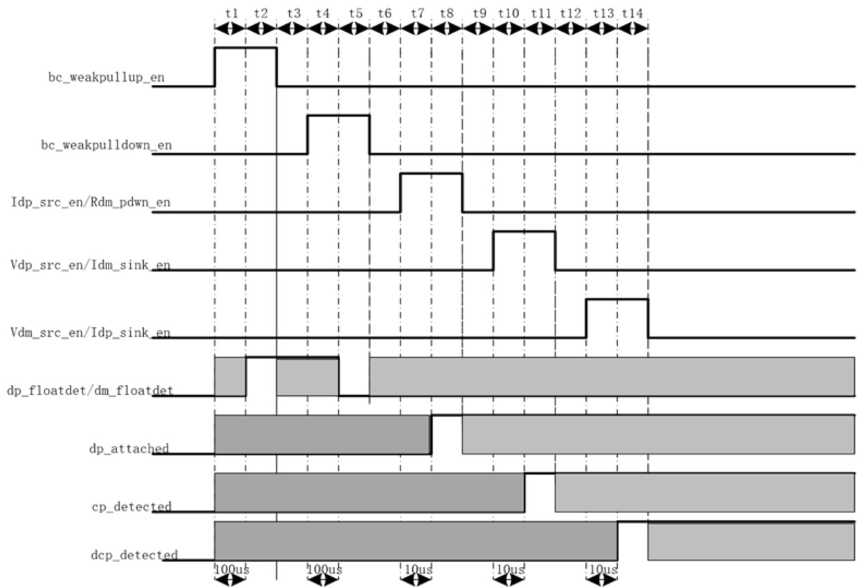
Figure 44. Battery Charging Sequence
