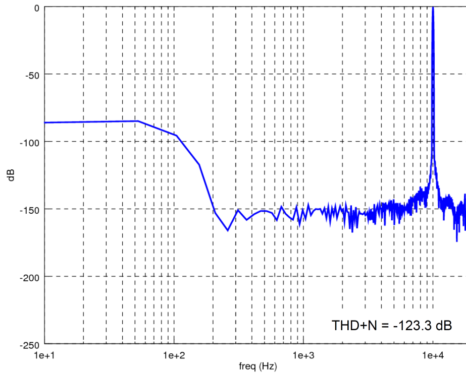
Figure 78. ASRC Performance Analysis - Test Case 4
