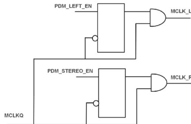
Figure 56. PDM Converter Core Local Clock Gating
