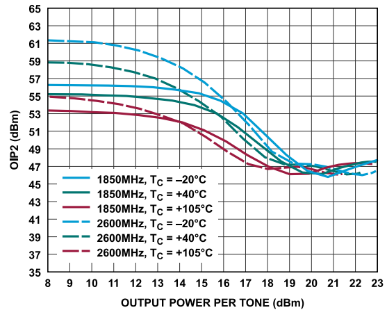
Figure 53. OIP2 vs. Output Power per Tone for Various Temperatures at 1850 MHz and 2600 MHz
