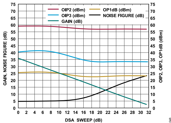
Figure 59. Gain, Noise Figure, OIP2, OIP3, OP1dB vs. DSA Sweep, Frequency = 2600 MHz
