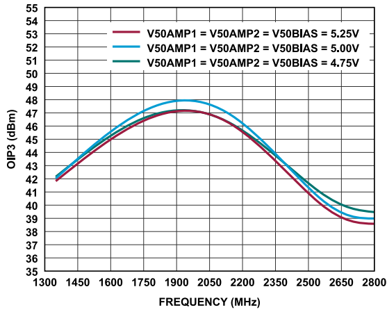
Figure 46. OIP3 vs. Frequency for Various Supplies
