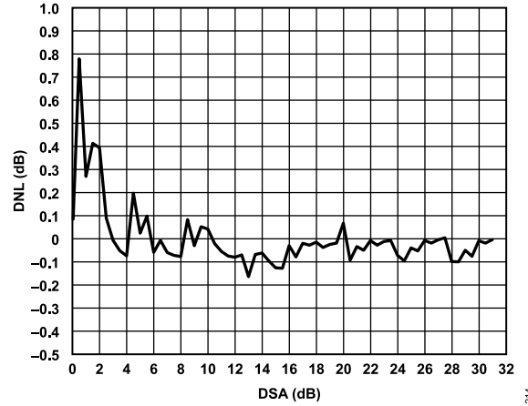
Figure 114. DSA Gain Step Error; Frequency = 4700 MHz
