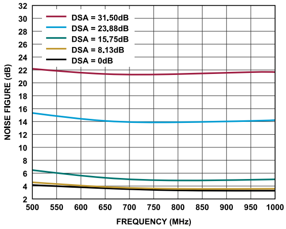
Figure 28. Noise Figure vs. Frequency at Various DSA Values
