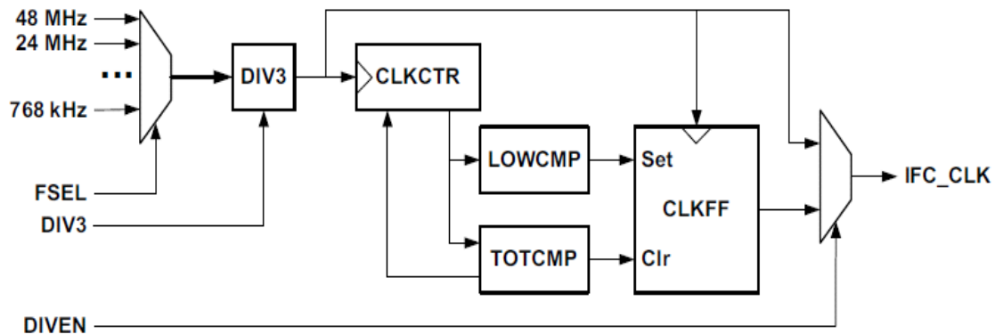
Figure 30. IO_CLK Generation
