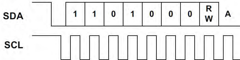
Figure 6-6: I 2 C 7-bit Address Operation
