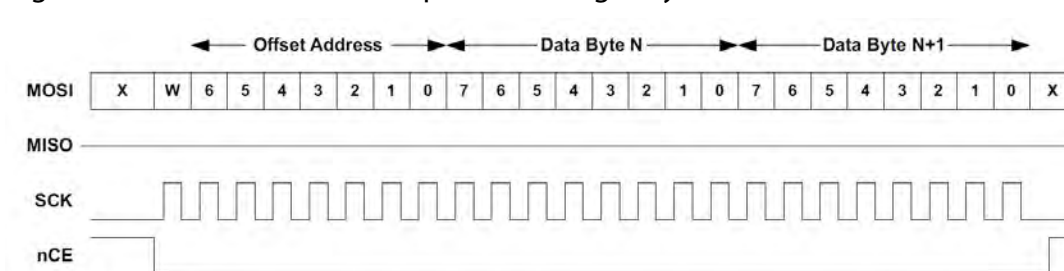
Figure 5-12: SPI Normal Write Operation (Single-byte Offset Address)
