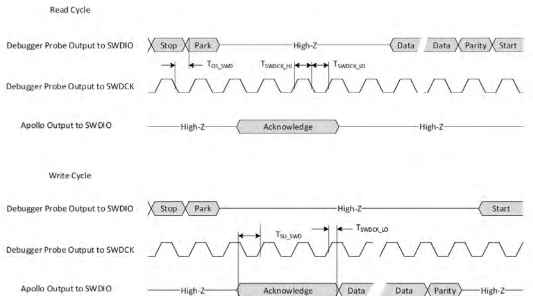
Figure 18-9: Serial Wire Debug Timing
