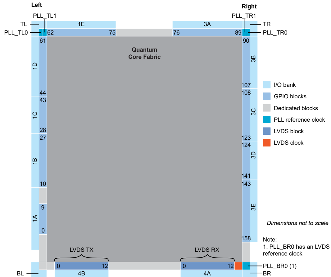
Figure 35: Floorplan Diagram for QFP144 Packages
