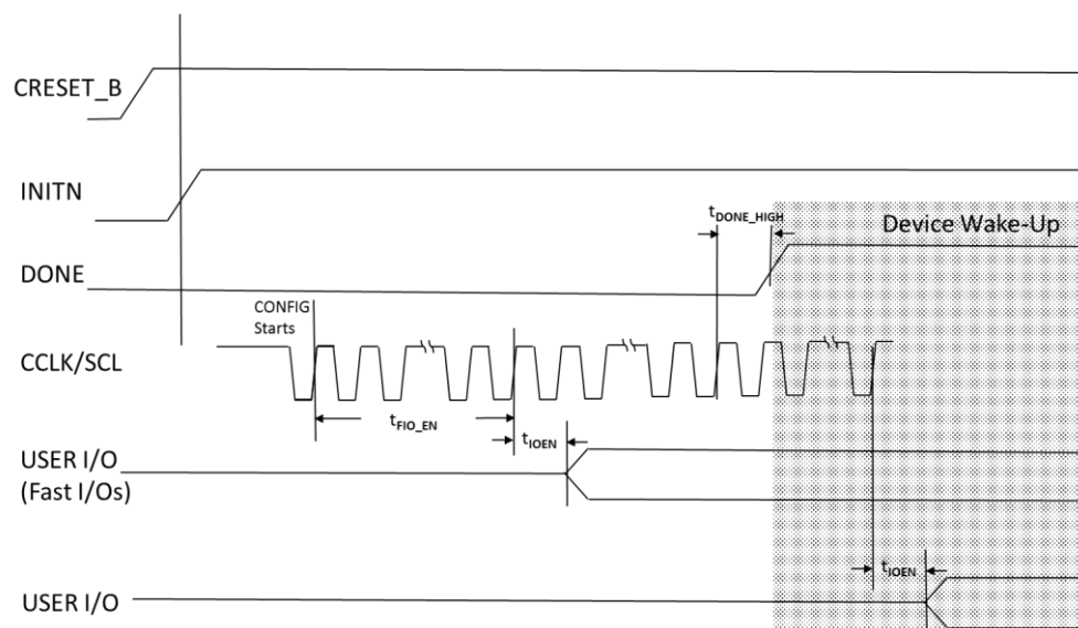
Figure 3.22. Slave SPI/I 2 C/I 3 C Wake-Up Timing
