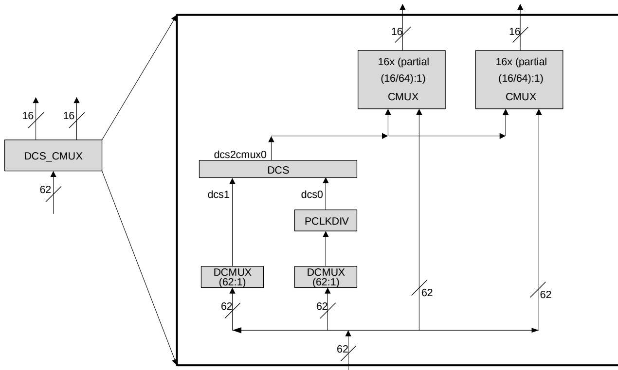
Figure 2.9. DCS_CMUX Diagram
