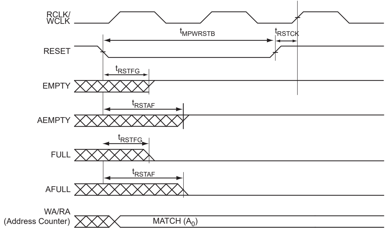
Figure 2-49 • FIFO Reset
