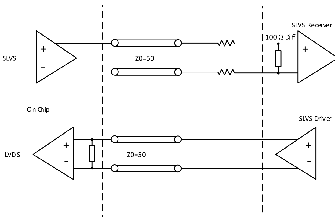
Figure 4.5. SLVS Interface
