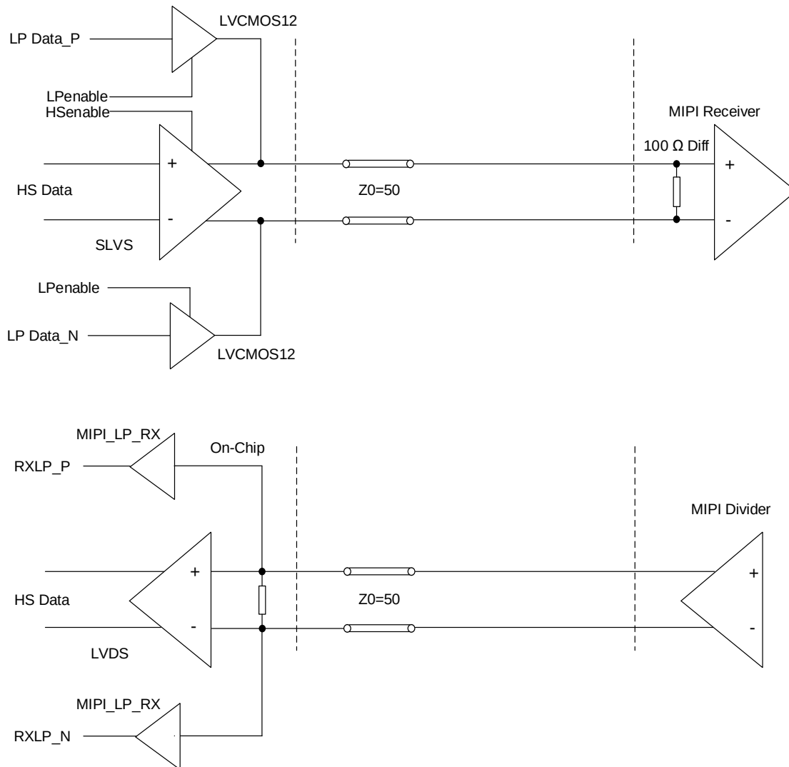
Figure 3.6. MIPI Interface
