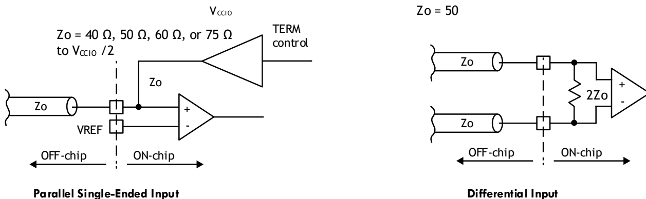
Figure 3.1. On-Chip Termination
