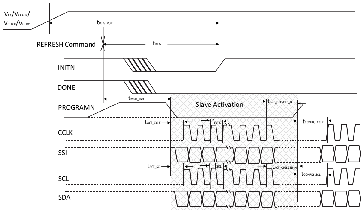
Figure 3.15. Target SPI/I2C/I3C POR/REFRESH Timing
