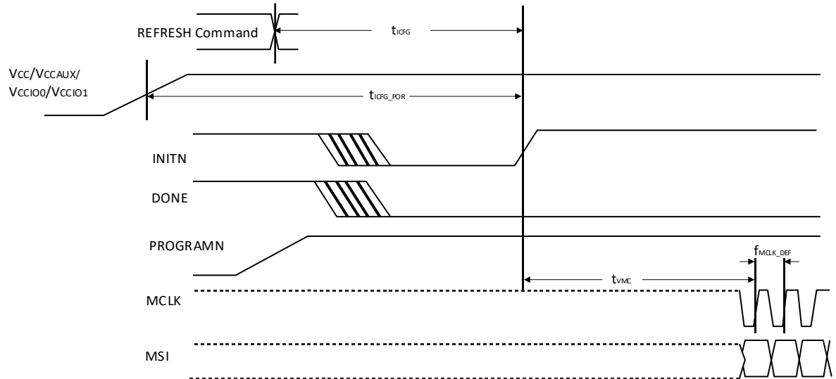
Figure 4.14. Controller SPI POR/REFRESH Timing
