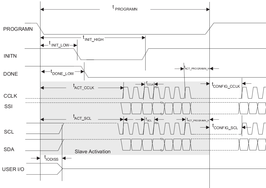
Figure 3.15. Slave SPI/I²C/I³C PROGRAMN Timing
