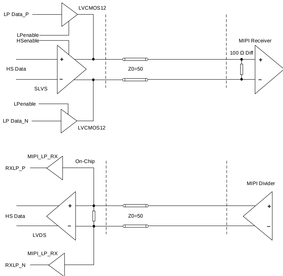
Figure 3.6. MIPI Interface
