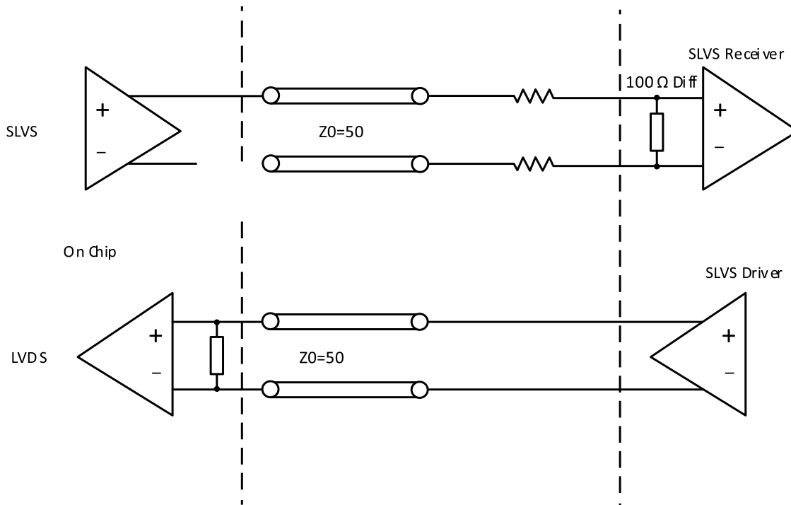
Figure 3.5. SLVS Interface
