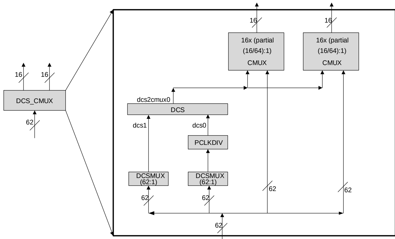
Figure 2.8. DCS_CMUX Diagram
