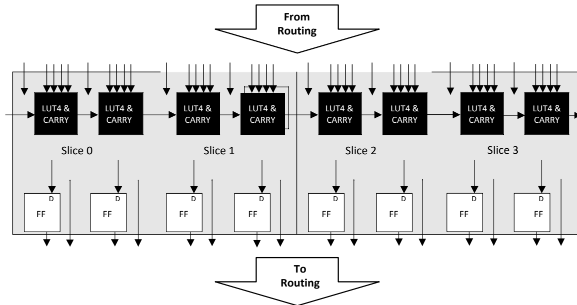
Figure 2.2. PFU Diagram
