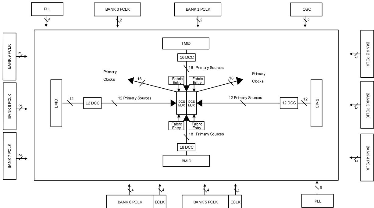
Figure 2.6. Clocking
