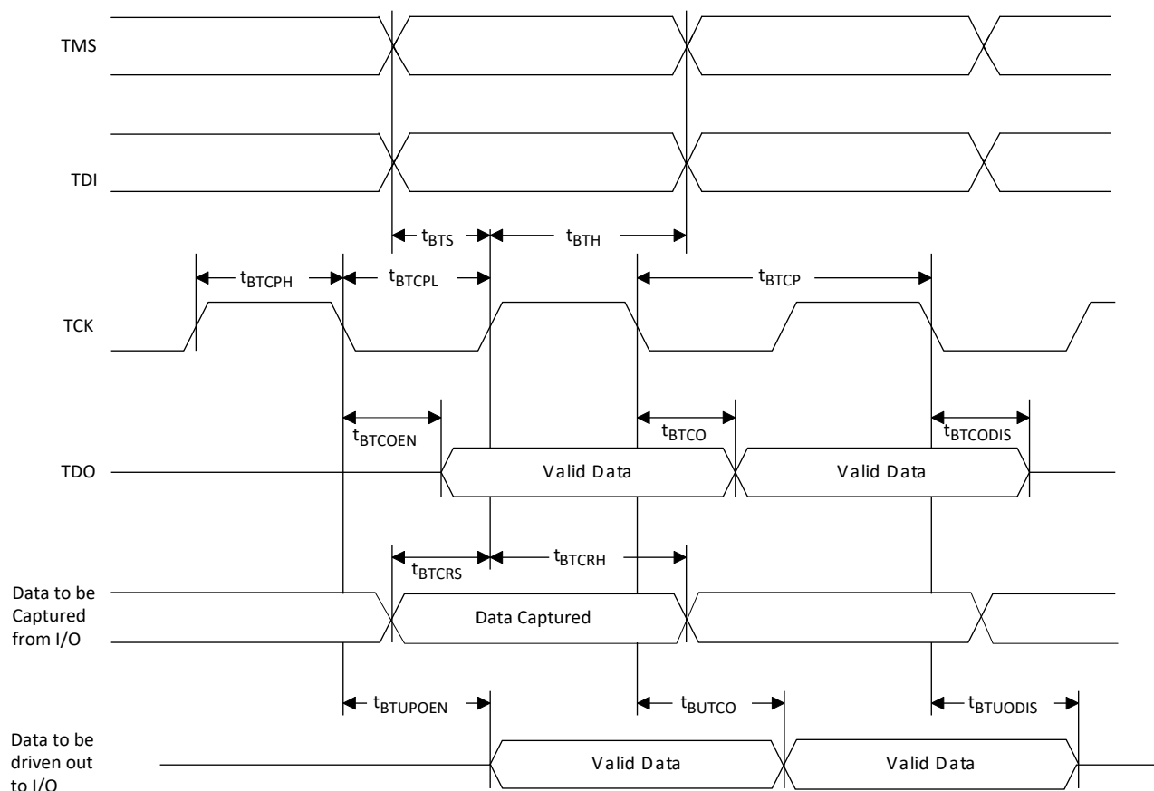
Figure 3.19. JTAG Port Timing Waveforms
