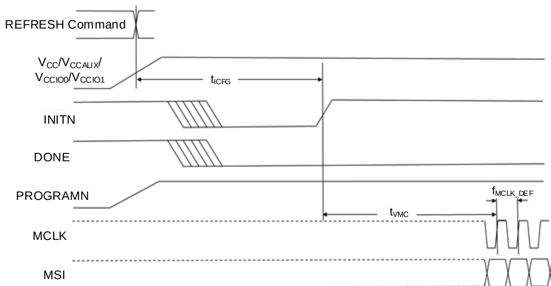
Figure 3.15. Master SPI POR/REFRESH Timing
