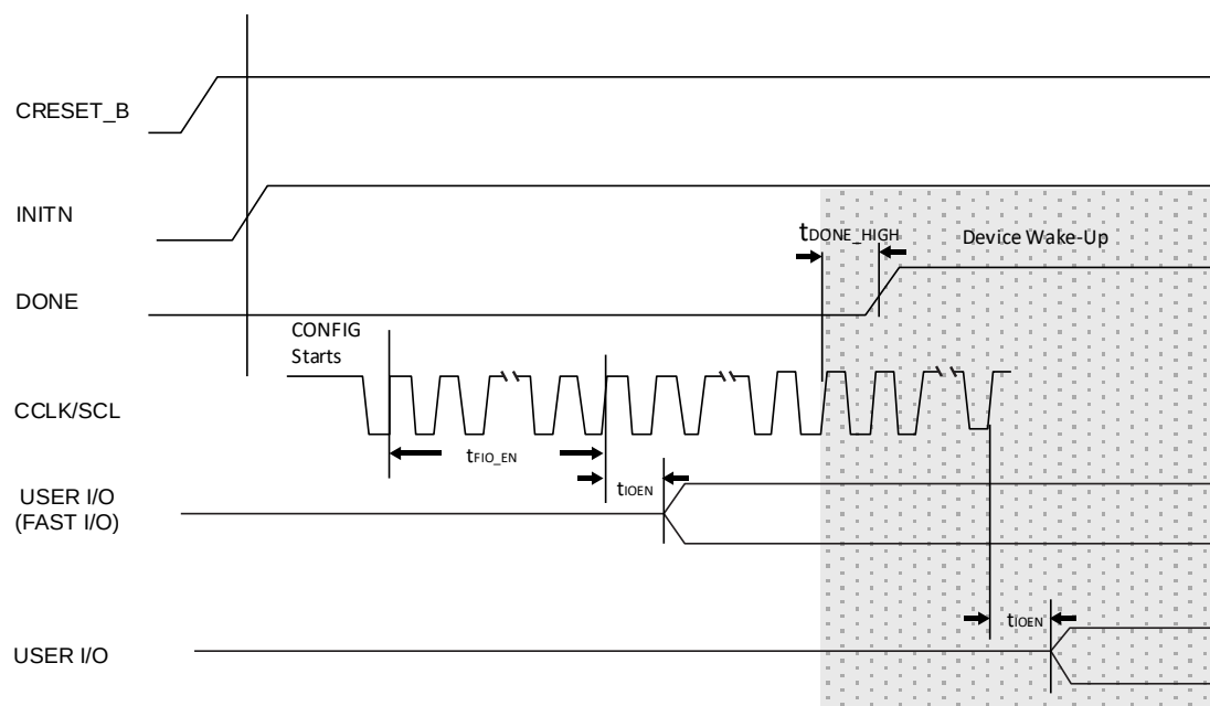
Figure 3.23. Slave SPI/I 2 C/I 3 C Wake-Up Timing
