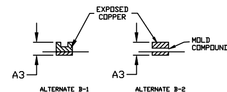
DETAIL B ALTERNATE CONSTRUCTION
