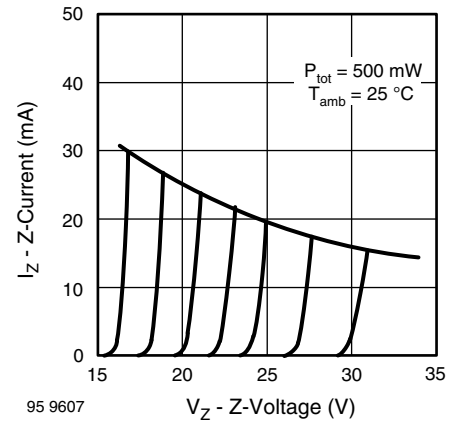
Fig. 8 - Typical Z-Current vs. Z-Voltage
