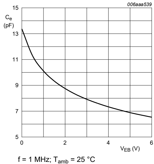
Fig. 8. Emitter capacitance as a function of emitter-base voltage; typical values
