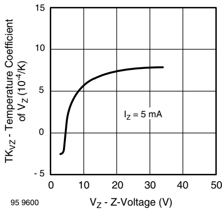
Fig. 4 - Typical Temperature Coefficient of V_Z vs. Z-Voltage
