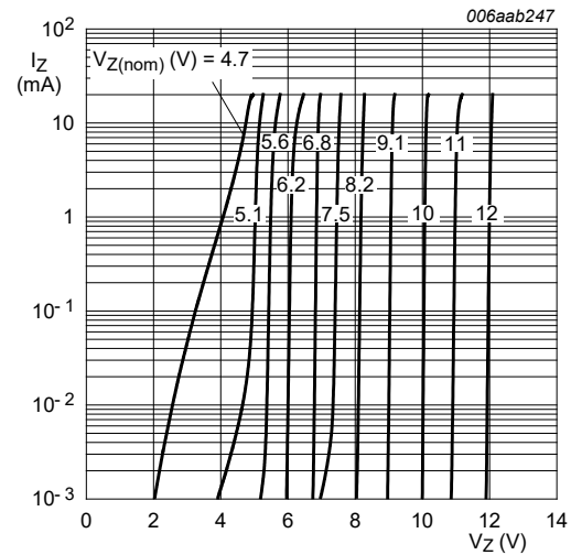
T_j = 25\text{ °C} V_Z = 4.7\text{ V} to 12\text{ V}
